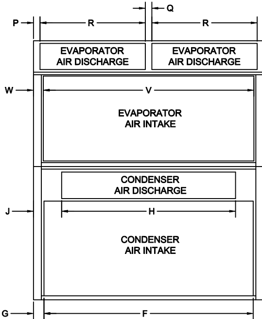
REAR VIEW
