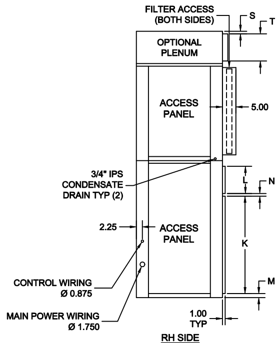
RH SIDE
