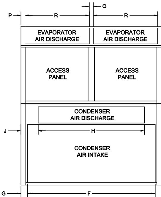
REAR VIEW
