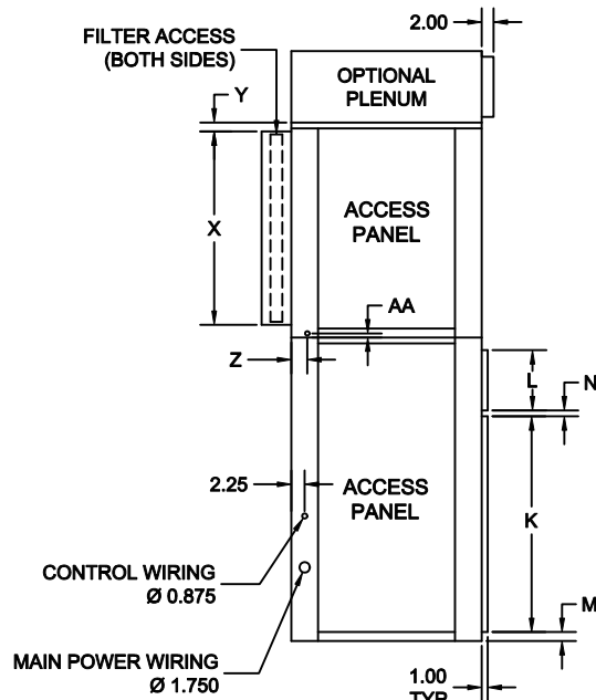
RH SIDE
