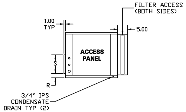
RH SIDE
