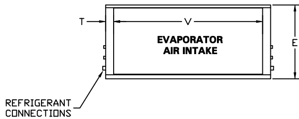
REAR VIEW
