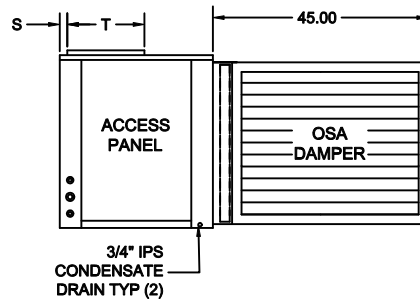
RH SIDE
