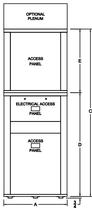
FRONT VIEW
