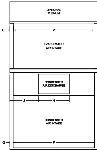
REAR VIEW
